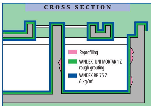
Sewage treatment plant Offenburg, Germany. Treated areas: external and internal waterproofing, base waterproofing; 3000 m 2 ; products used: VANDEX BB 75, VANDEX BB 75 Z, VANDEX MINERALIT, VANDEX UNI MORTAR 1 Z.
